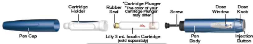
HumaPen Ergo™ II Pen Parts
